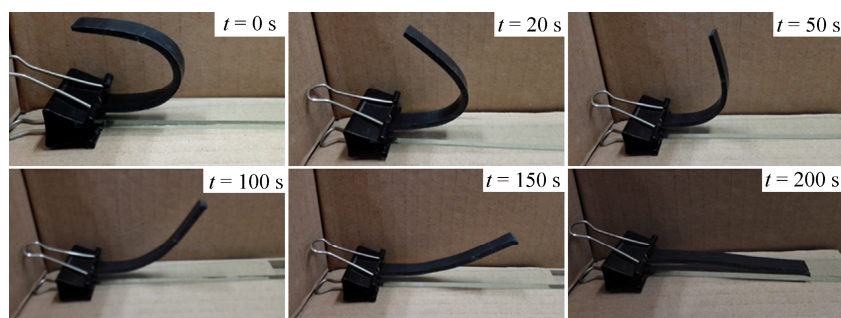
Fig. 7 Shape memory test of SCF/SBS/LLDPE composite with 6.0 wt% of SCF at 110 °C
