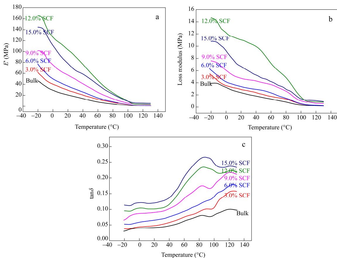
Fig. 4 Dynamic mechanical properties of the SCF/SBS/LLDPE composites: (a) E' , (b) loss modulus and (c) \tan\delta
