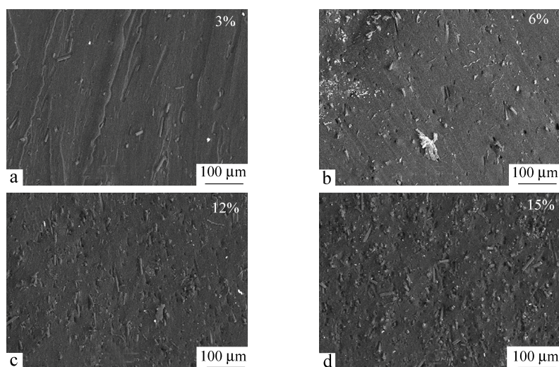
Fig. 5 SEM images of the composites with different SCF contents: (a) 3%, (b) 6%, (c) 12% and (d) 15%
